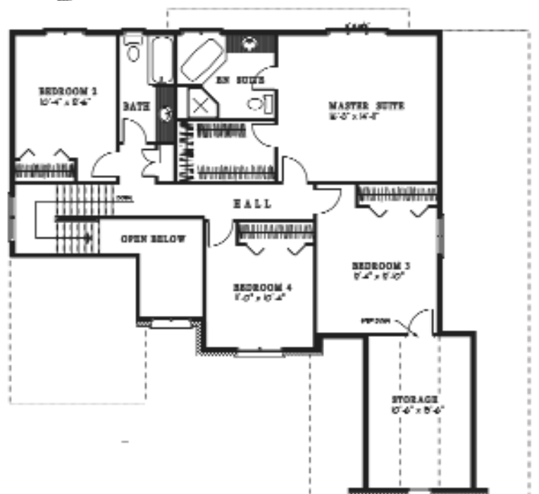
Upper Floor Plan 1,398 SQ.FT. plus 80 SQ.FT. of open space
