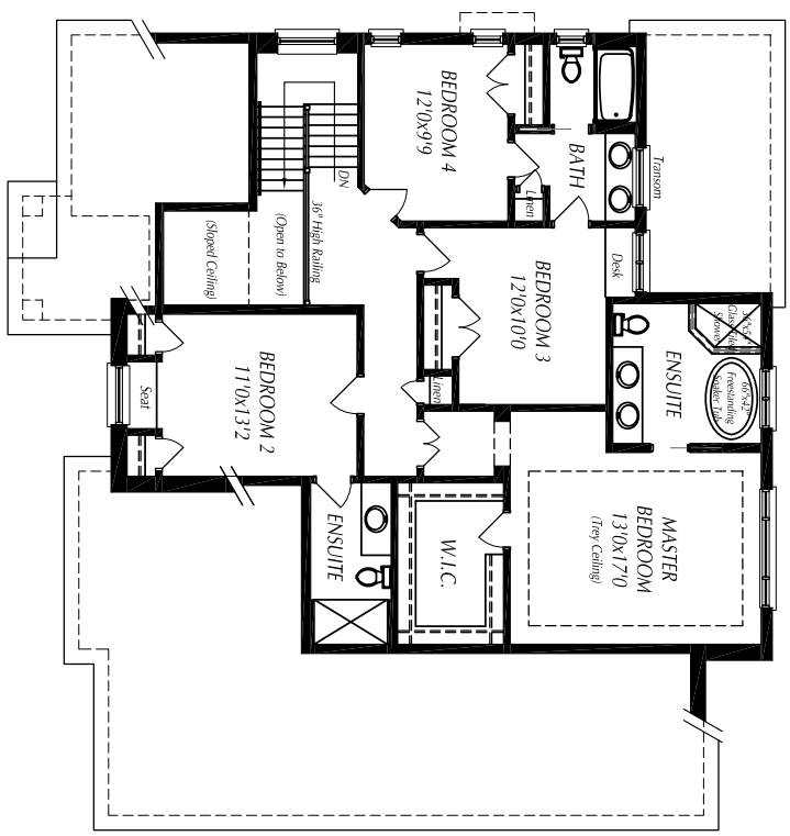
SECOND FLOOR PLAN 1370 sq ft + 67 sq ft open space
