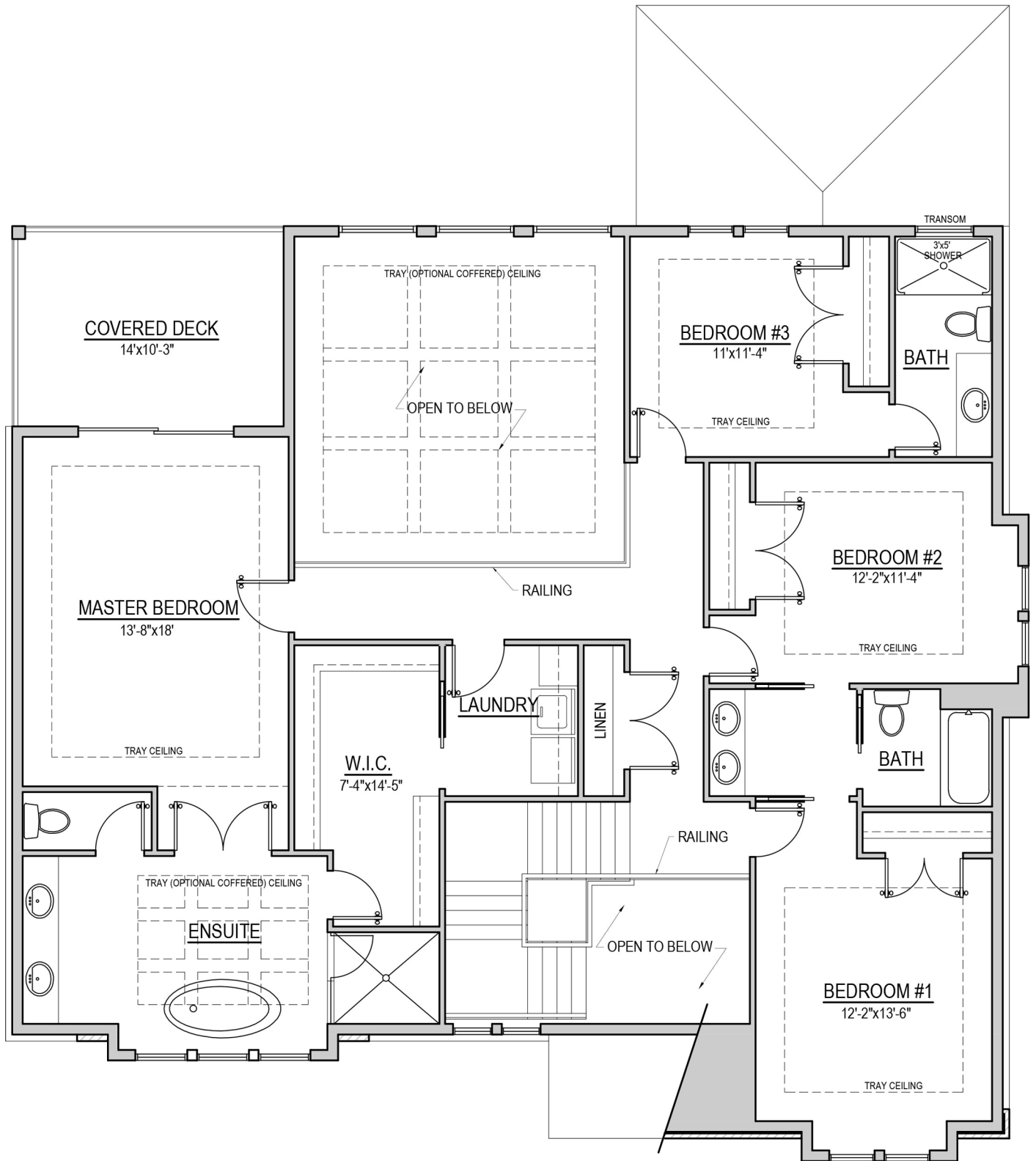
SECOND FLOOR PLAN - 1,621 SQ. FT. + 460 SQ. FT. OPEN SPACE
