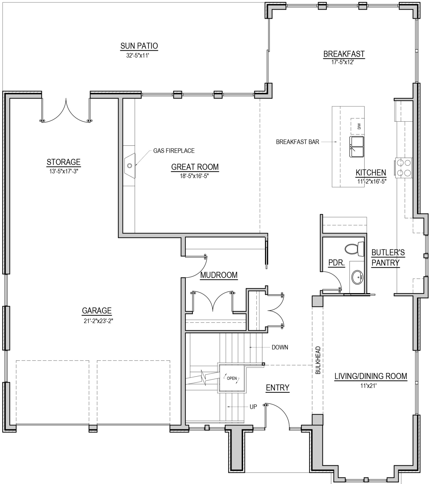
FIRST FLOOR PLAN - 1,690 SQ. FT. + 790 SQ. FT. GARAGE
